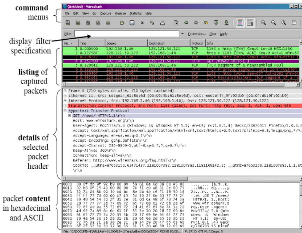
Figure 8: Wireshark Graphical User Interface on Microsoft Windows
